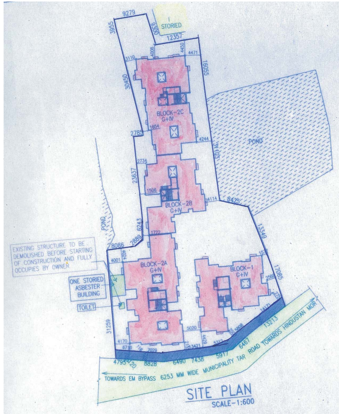
SITE PLAN
